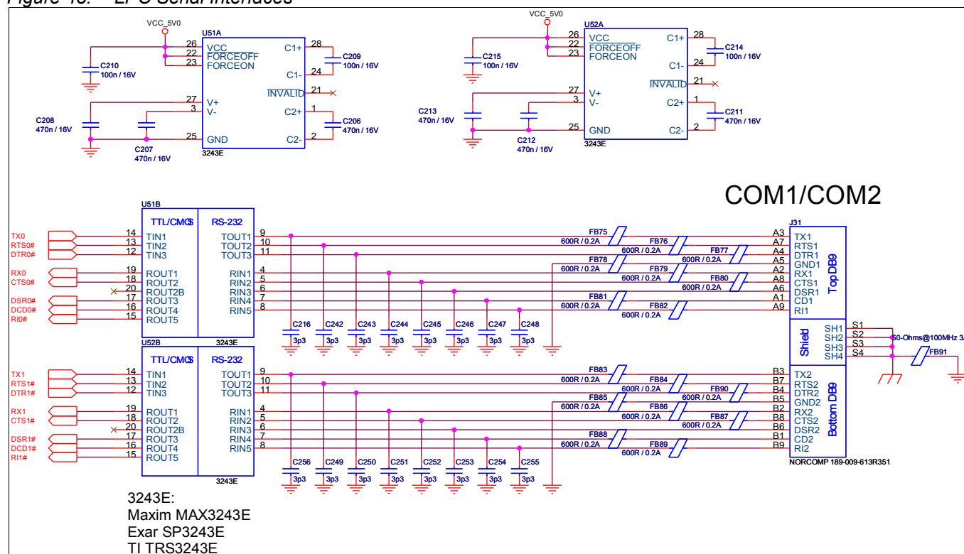
Figure 45: LPC Serial Interfaces
