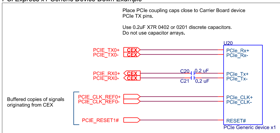
Figure 9: PCI Express x1 Generic Device Down Example
