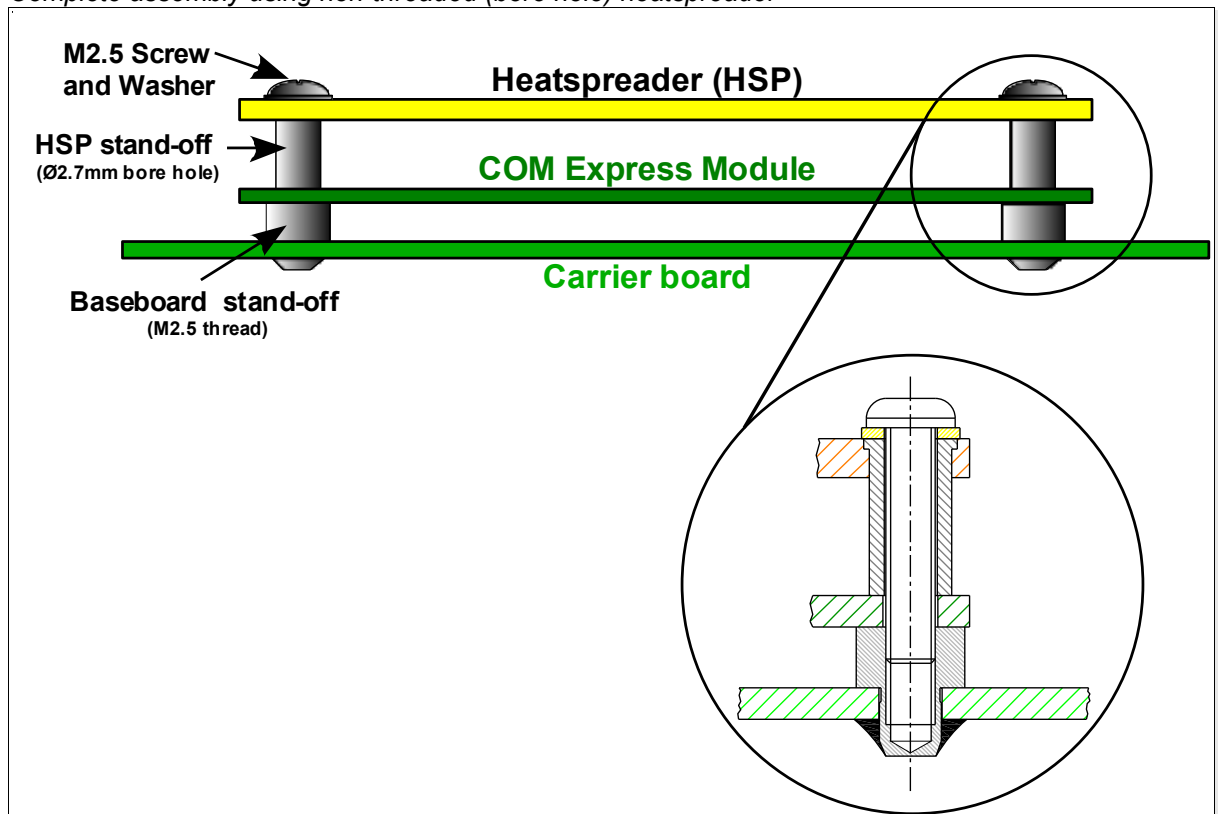
Figure 76: Complete assembly using non-threaded (bore hole) heatspreader
