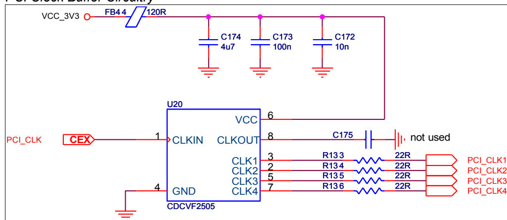
Figure 61: PCI Clock Buffer Circuitry
