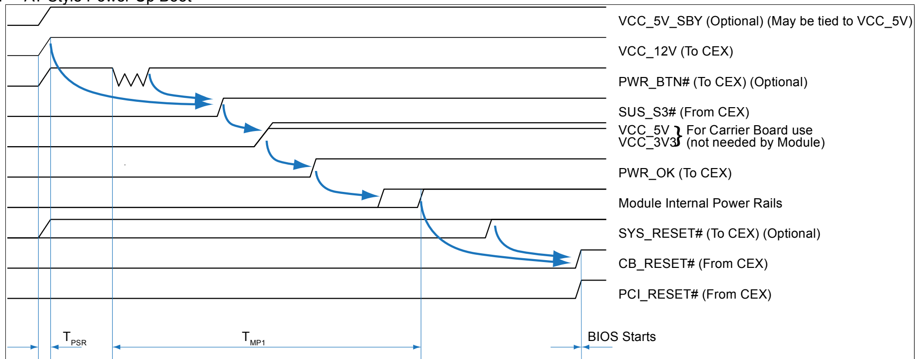
Figure 65: AT Style Power Up Boot
