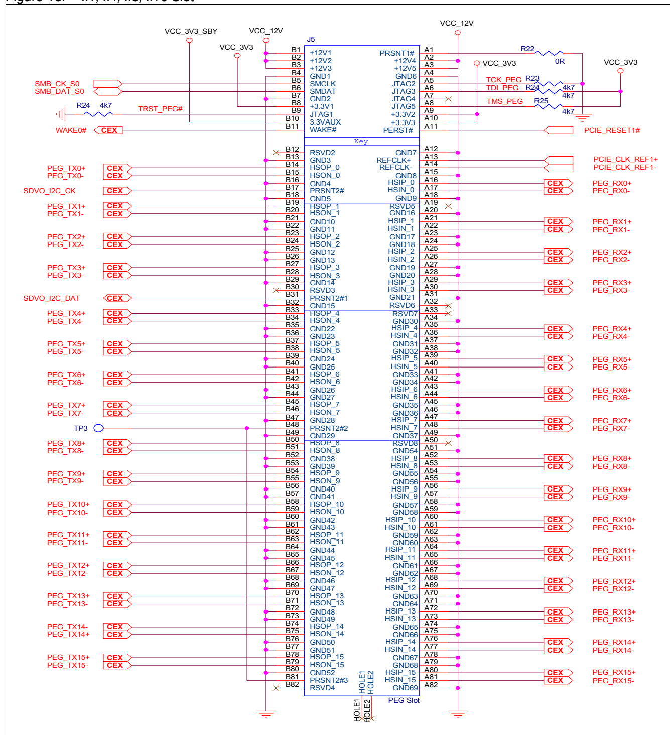
Figure 18: x1, x4, x8, x16 Slot
