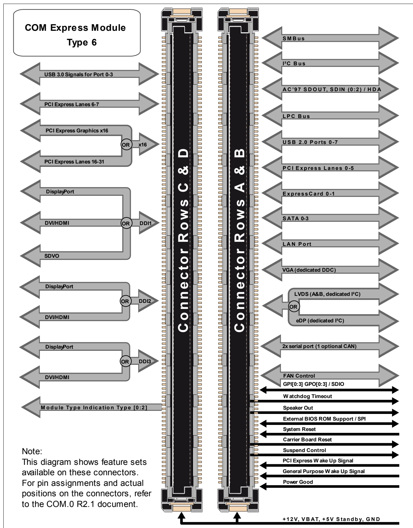
Figure 4: COM Express Type 6 Connector Layout
