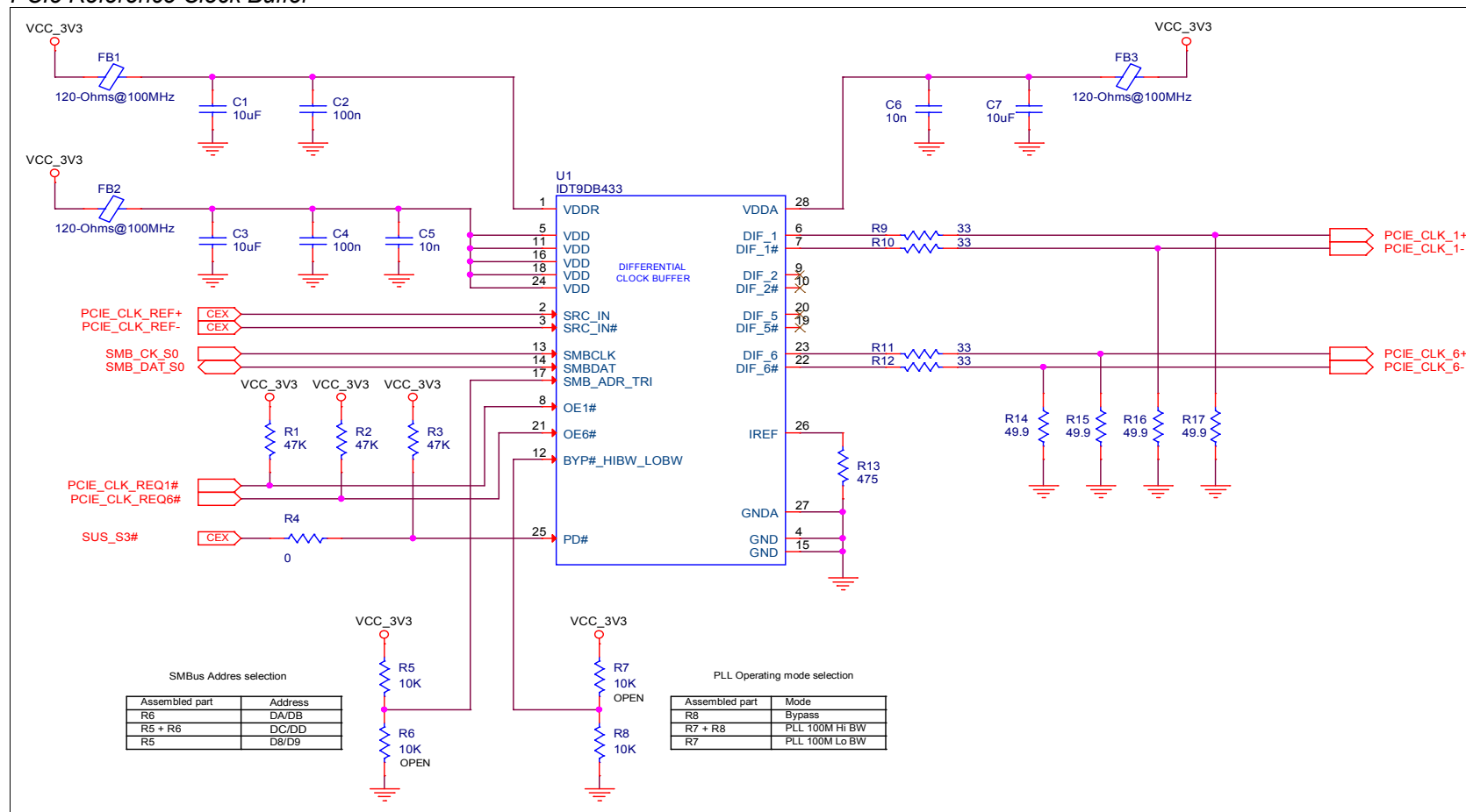
Figure 6: PCIe Reference Clock Buffer
