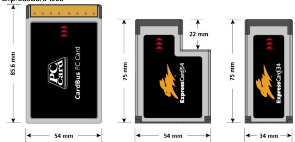
Figure 15: ExpressCard Size
