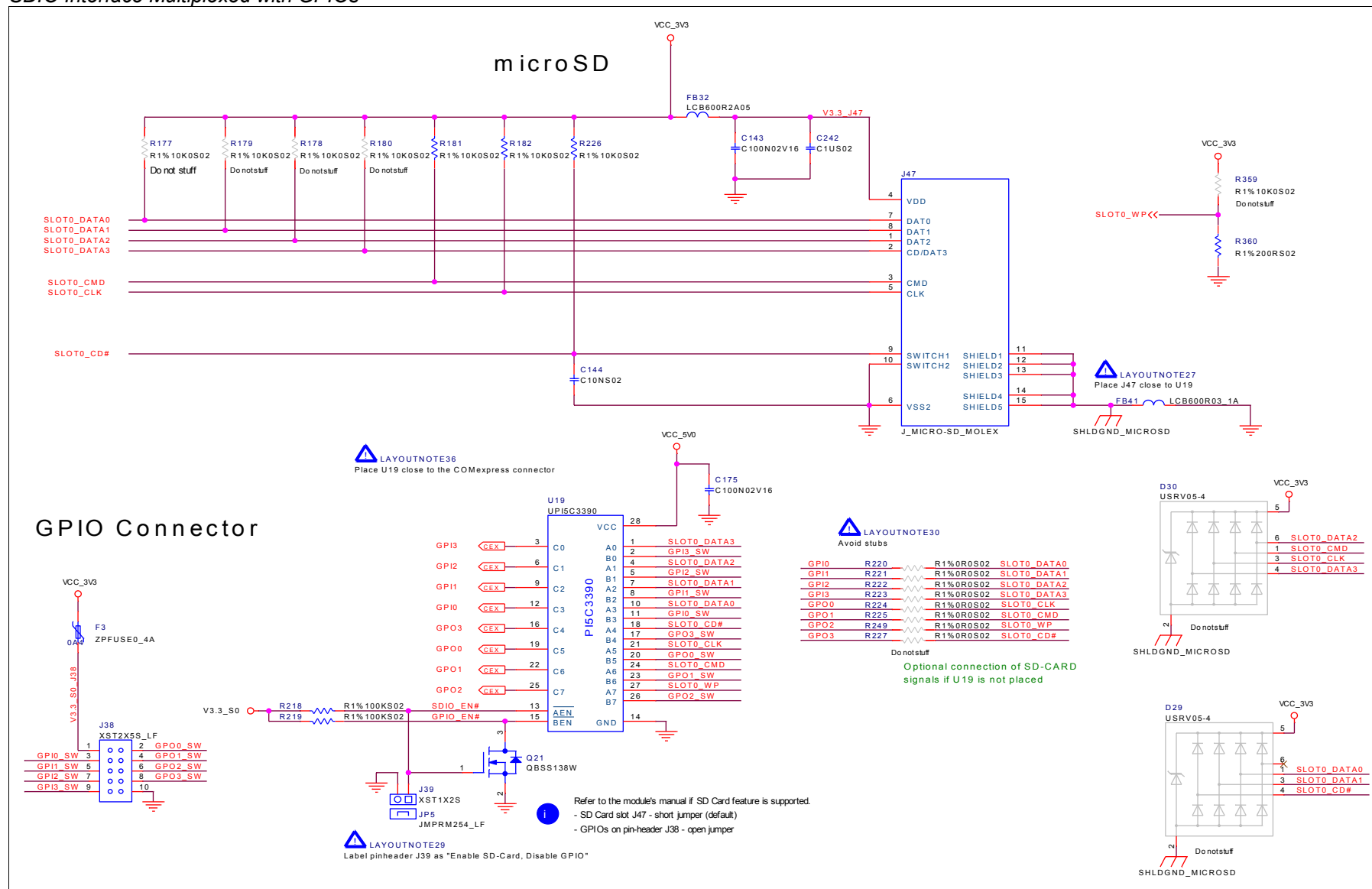
Figure 56: SDIO Interface Multiplexed with GPIOs
