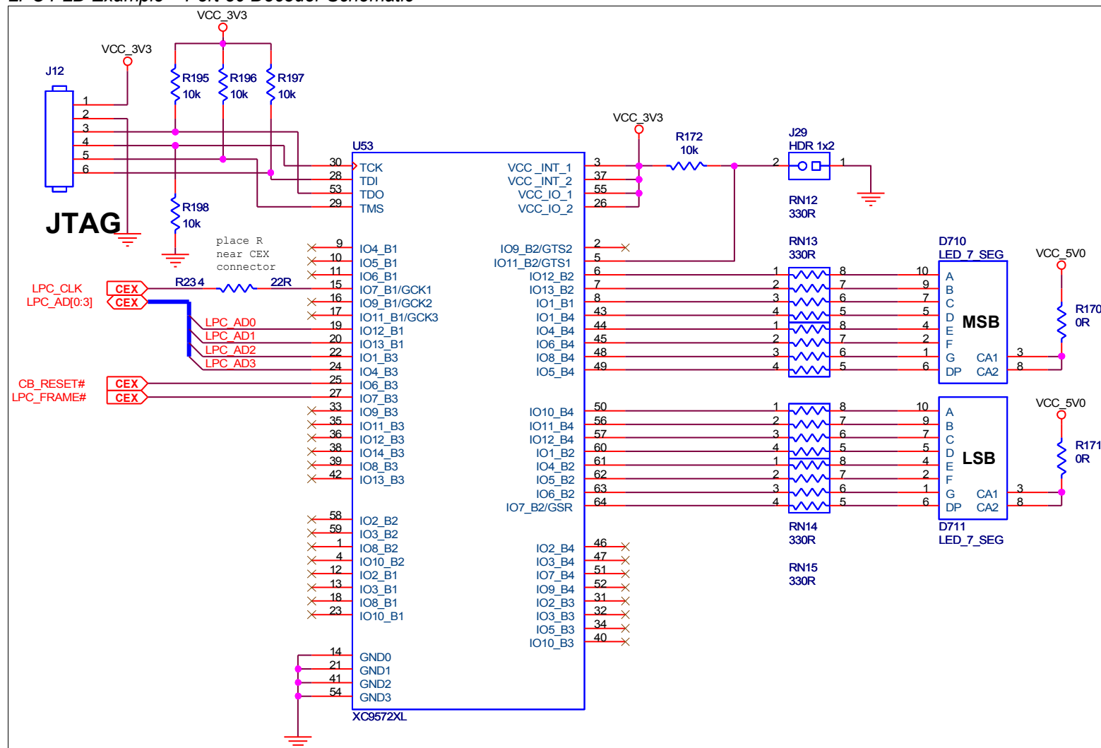
Figure 43: LPC PLD Example – Port 80 Decoder Schematic
