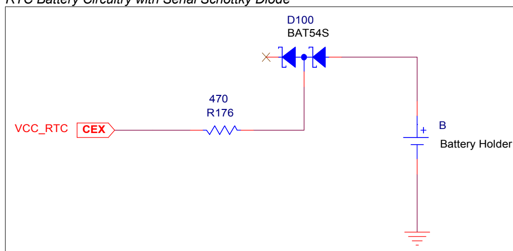
Figure 53: RTC Battery Circuitry with Serial Schottky Diode
