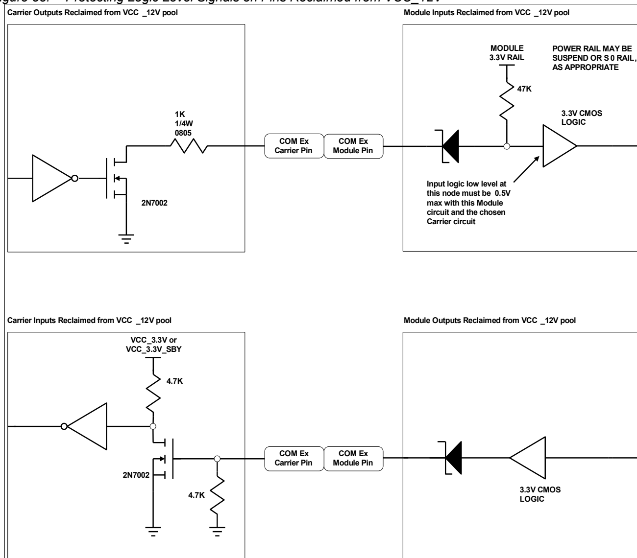
Figure 58: Protecting Logic Level Signals on Pins Reclaimed from VCC_12V
