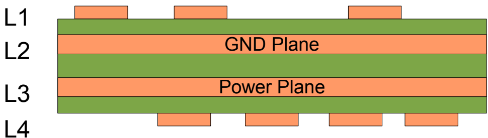
Figure 68: Four-Layer Stack-up
