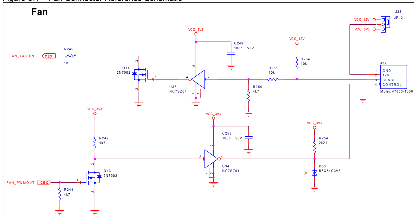
Figure 57: Fan Connector Reference Schematic
