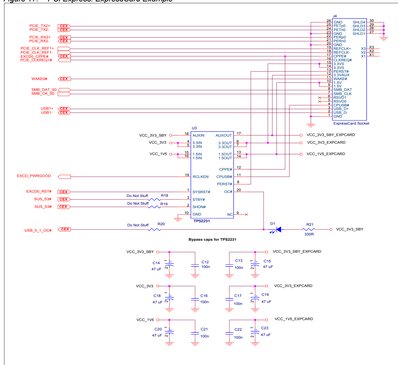
Figure 17: PCI Express: ExpressCard Example
