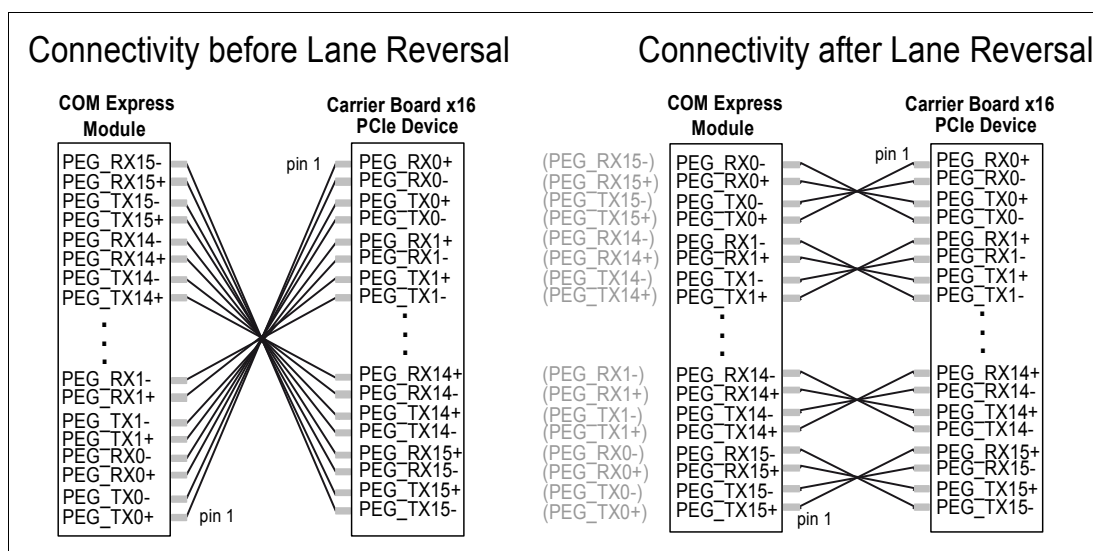
Figure 19: PEG Lane Reversal Mode
