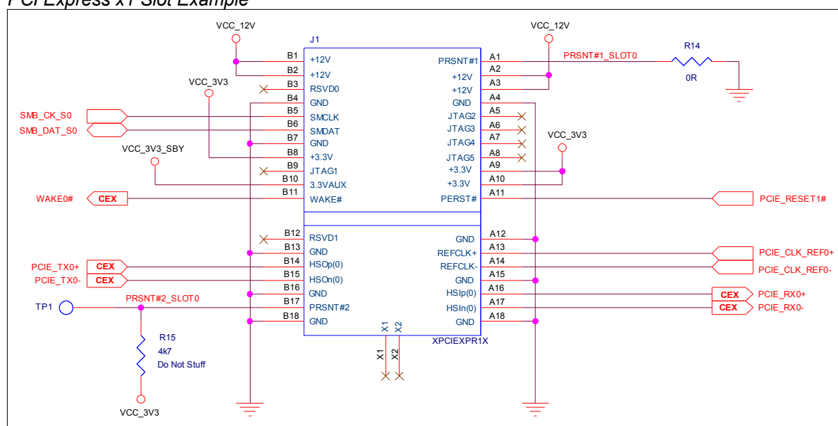
Figure 7: PCI Express x1 Slot Example
