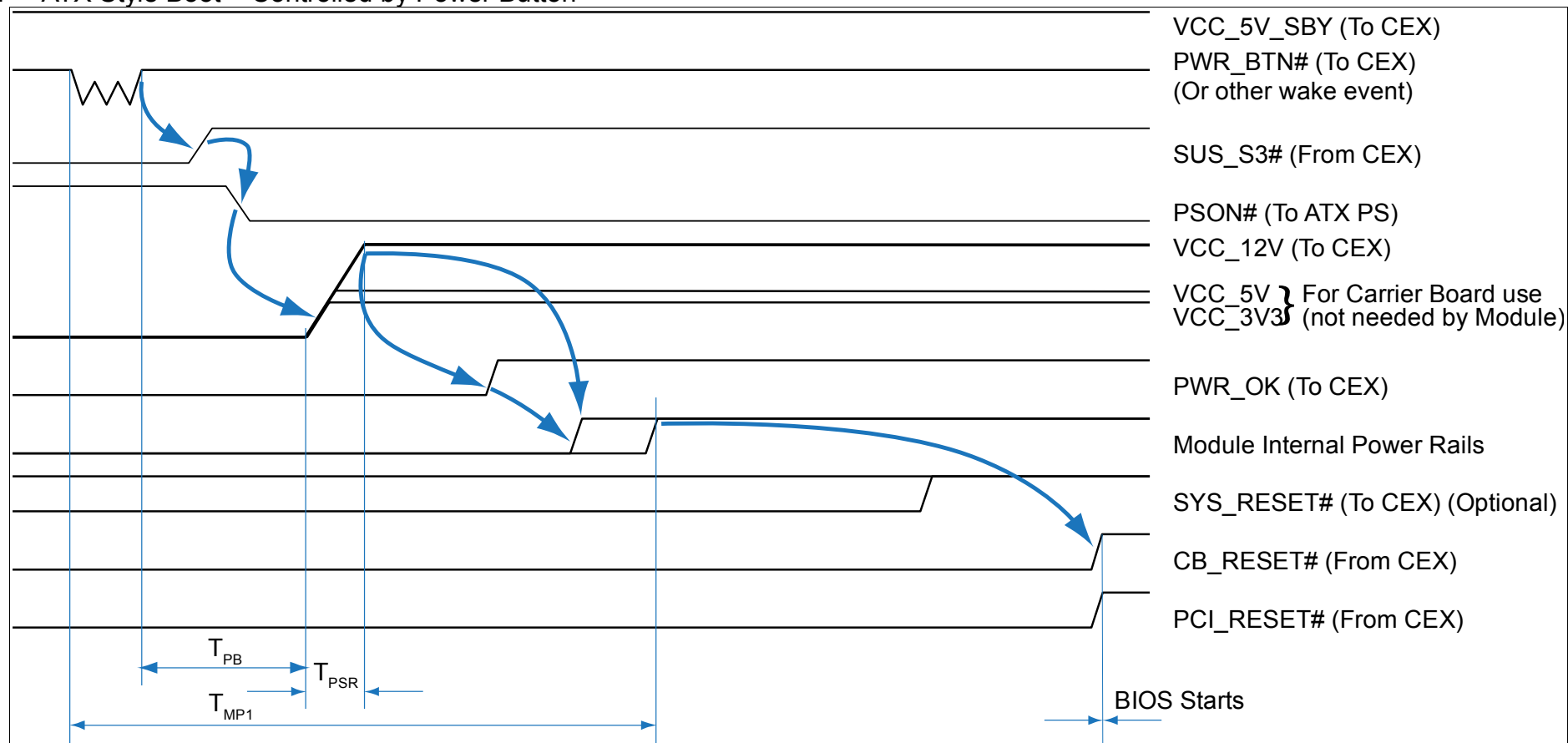
Figure 64: ATX Style Boot – Controlled by Power Button
