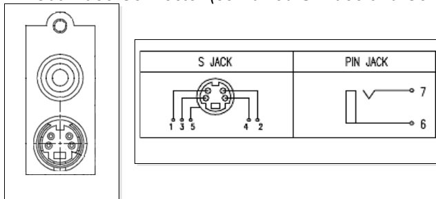
Figure 78: TV-Out Video Connector (combined S-Video and Composite)
