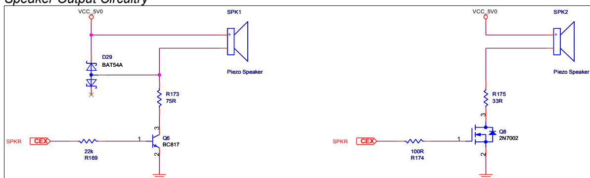
Figure 52: Speaker Output Circuitry
