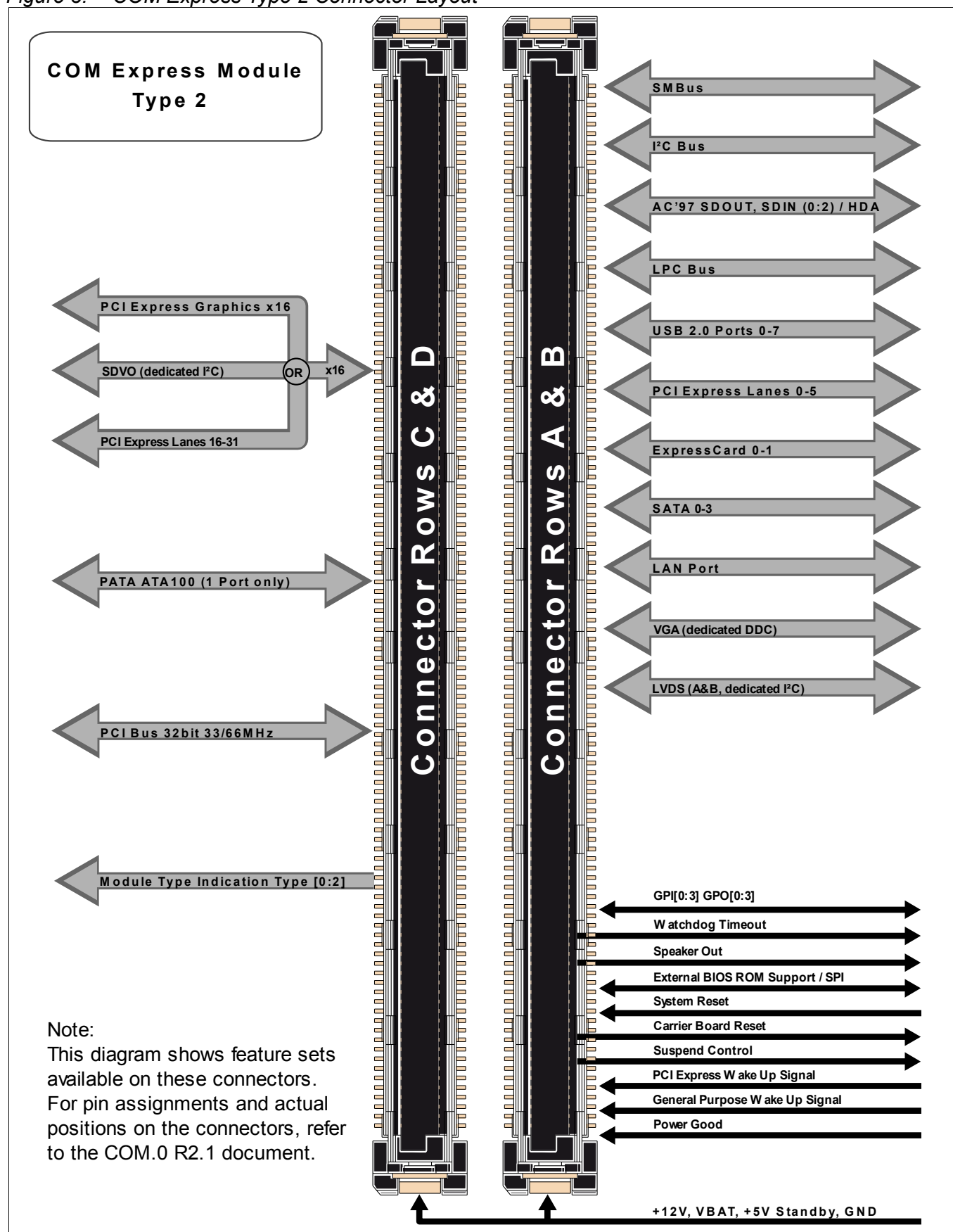
Figure 3: COM Express Type 2 Connector Layout
