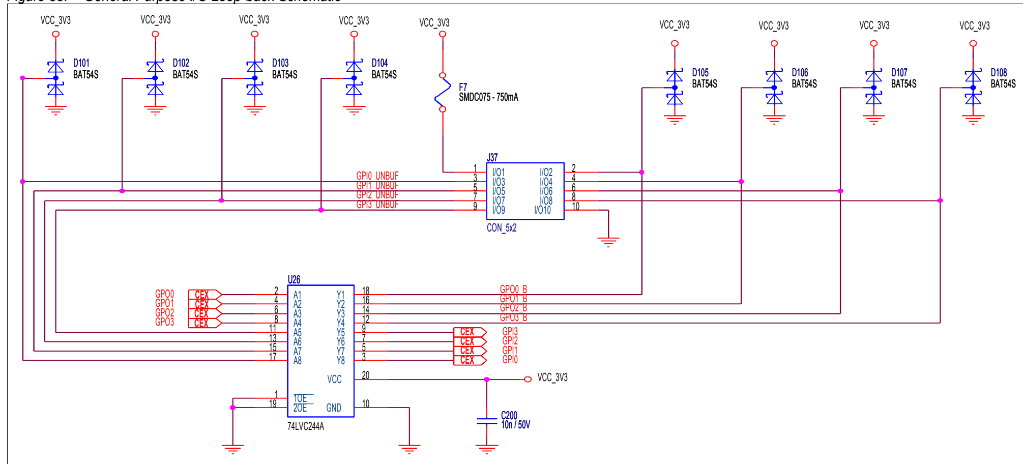
Figure 55: General Purpose I/O Loop-back Schematic
