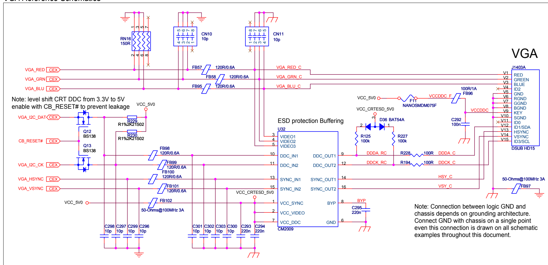
Figure 37: VGA Reference Schematics
