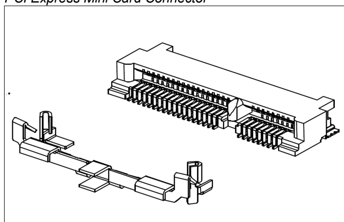
Figure 12: PCI Express Mini Card Connector
