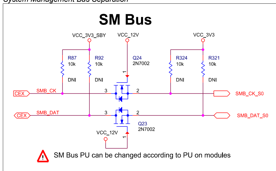
Figure 48: System Management Bus Separation
