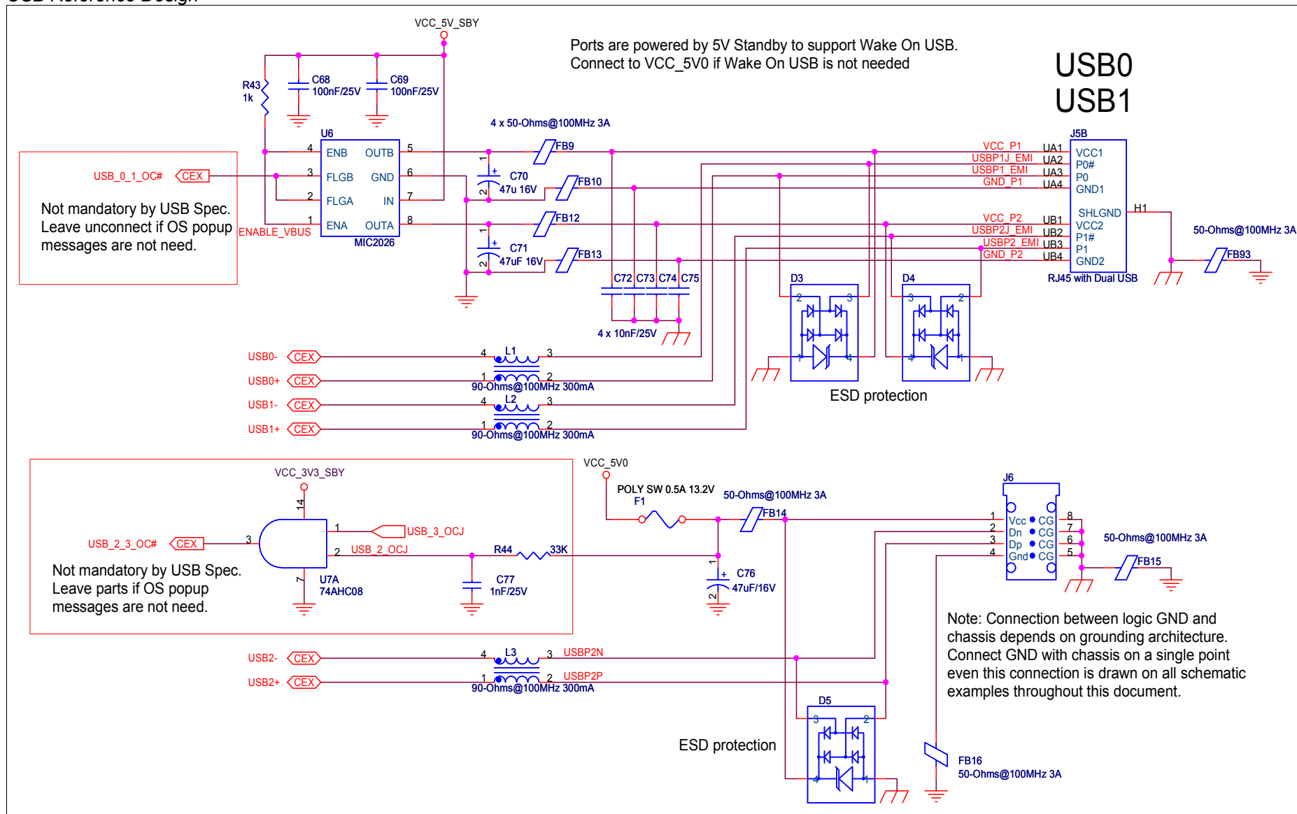
Figure 29: USB Reference Design
