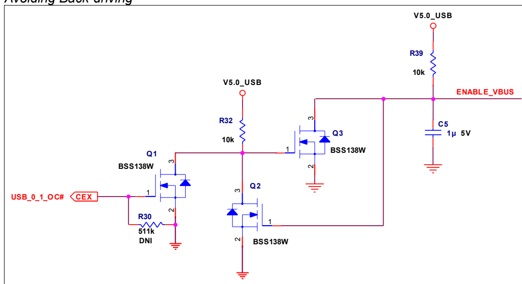
Figure 32: Avoiding Back-driving
