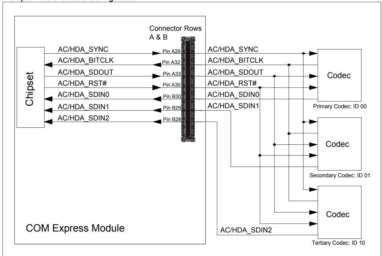
Figure 38: Multiple Audio Codec Configuration
