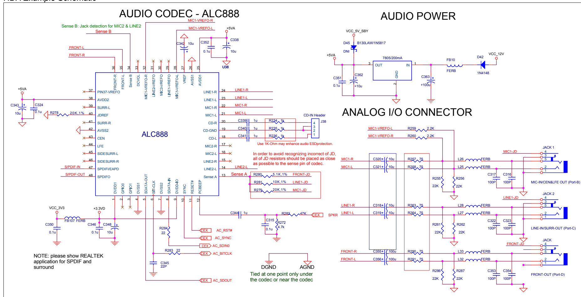
Figure 39: HDA Example Schematic
