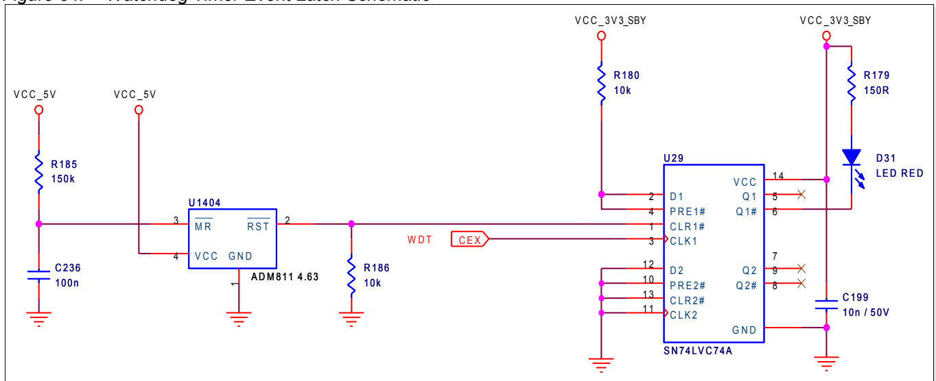
Figure 54: Watchdog Timer Event Latch Schematic
