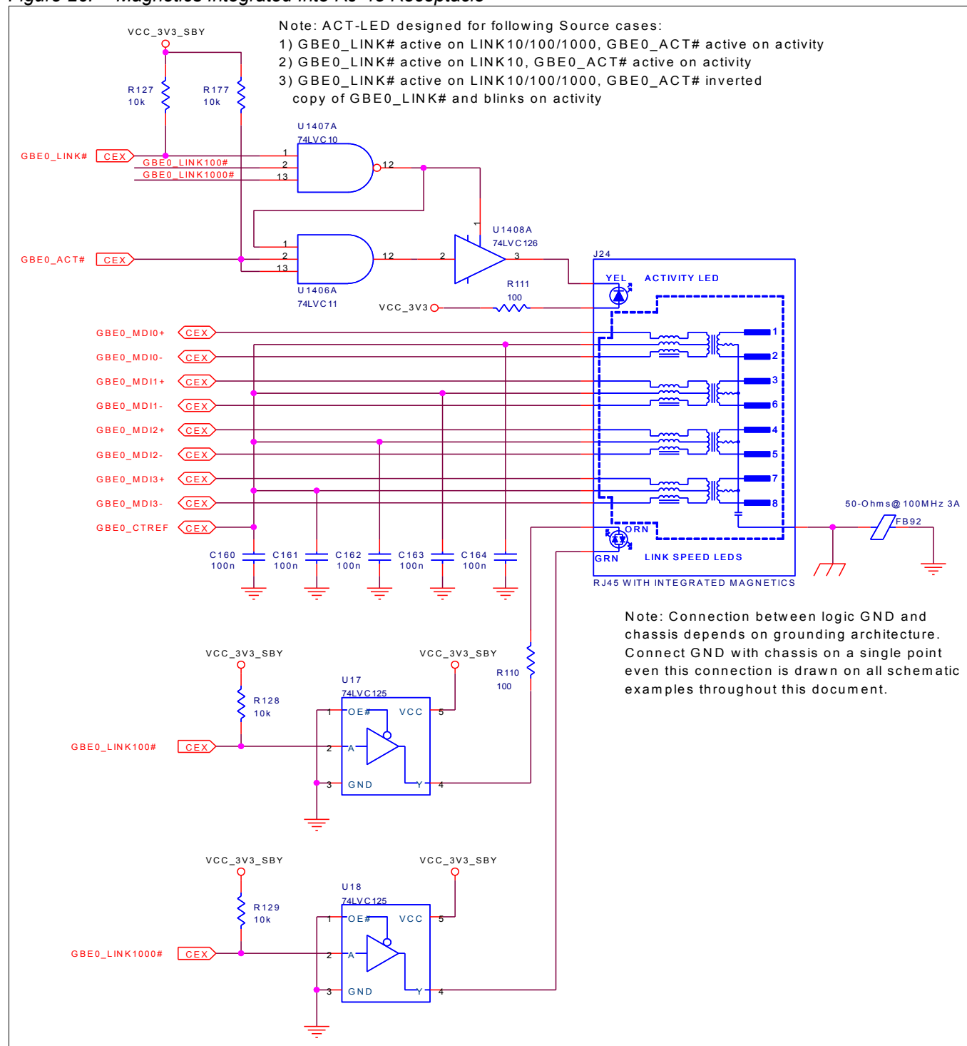
Figure 26: Magnetics Integrated Into RJ-45 Receptacle
