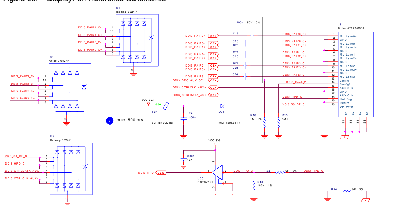
Figure 20: DisplayPort Reference Schematics
