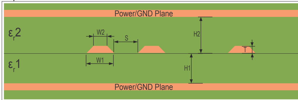
Figure 72: Strip Line Cross Section
