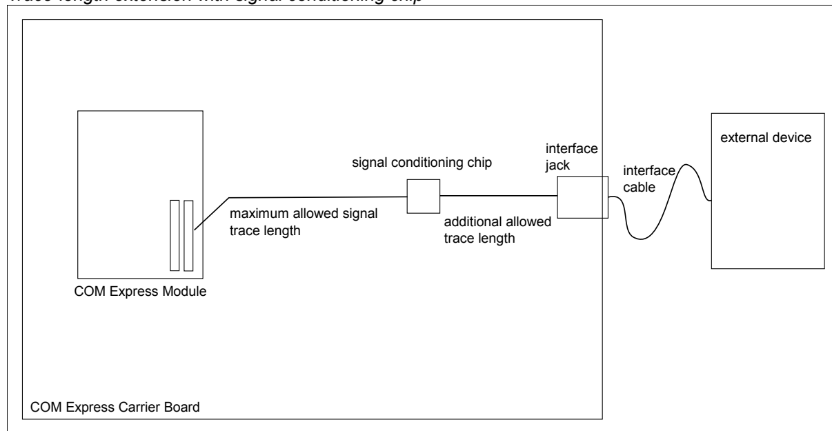
Figure 73: Trace-length extension with signal conditioning chip
