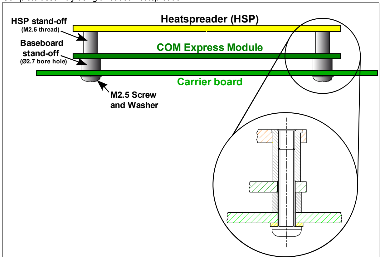
Figure 77: Complete assembly using threaded heatspreader
