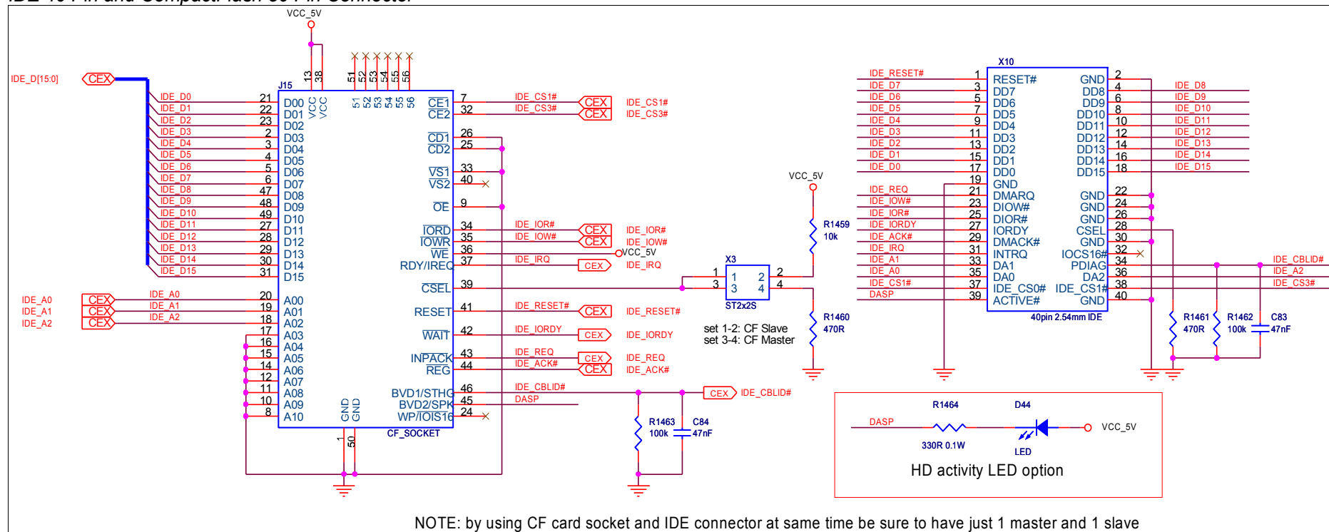
Figure 63: IDE 40 Pin and CompactFlash 50 Pin Connector
