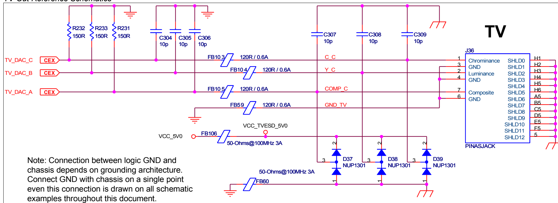
Figure 79: TV-Out Reference Schematics
