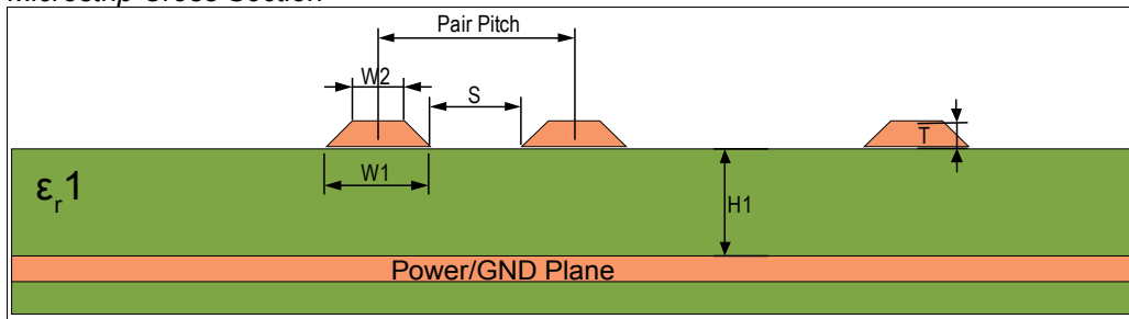
Figure 71: Microstrip Cross Section
