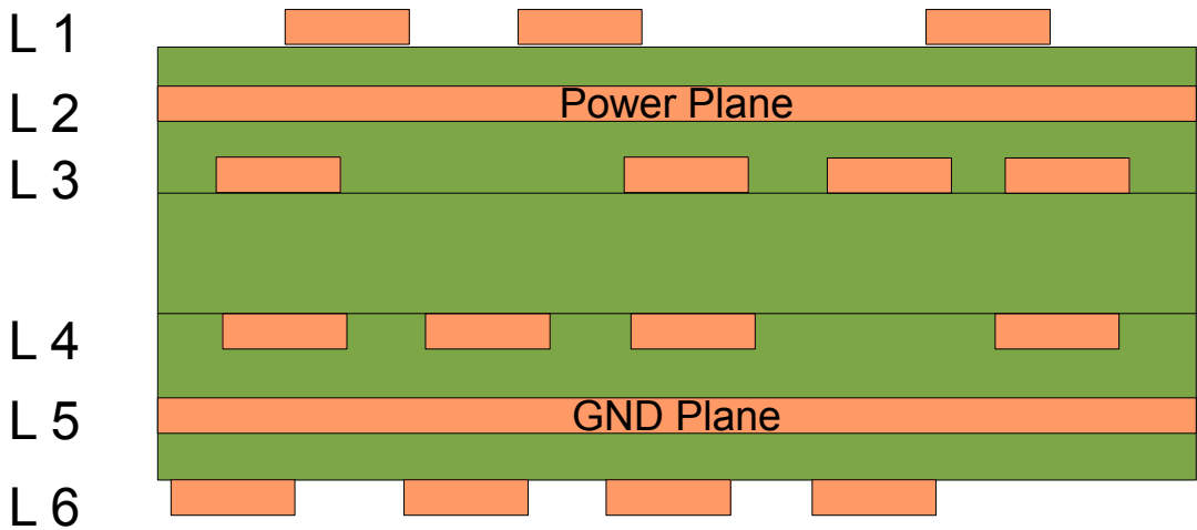
Figure 69: Six-Layer Stack-up
