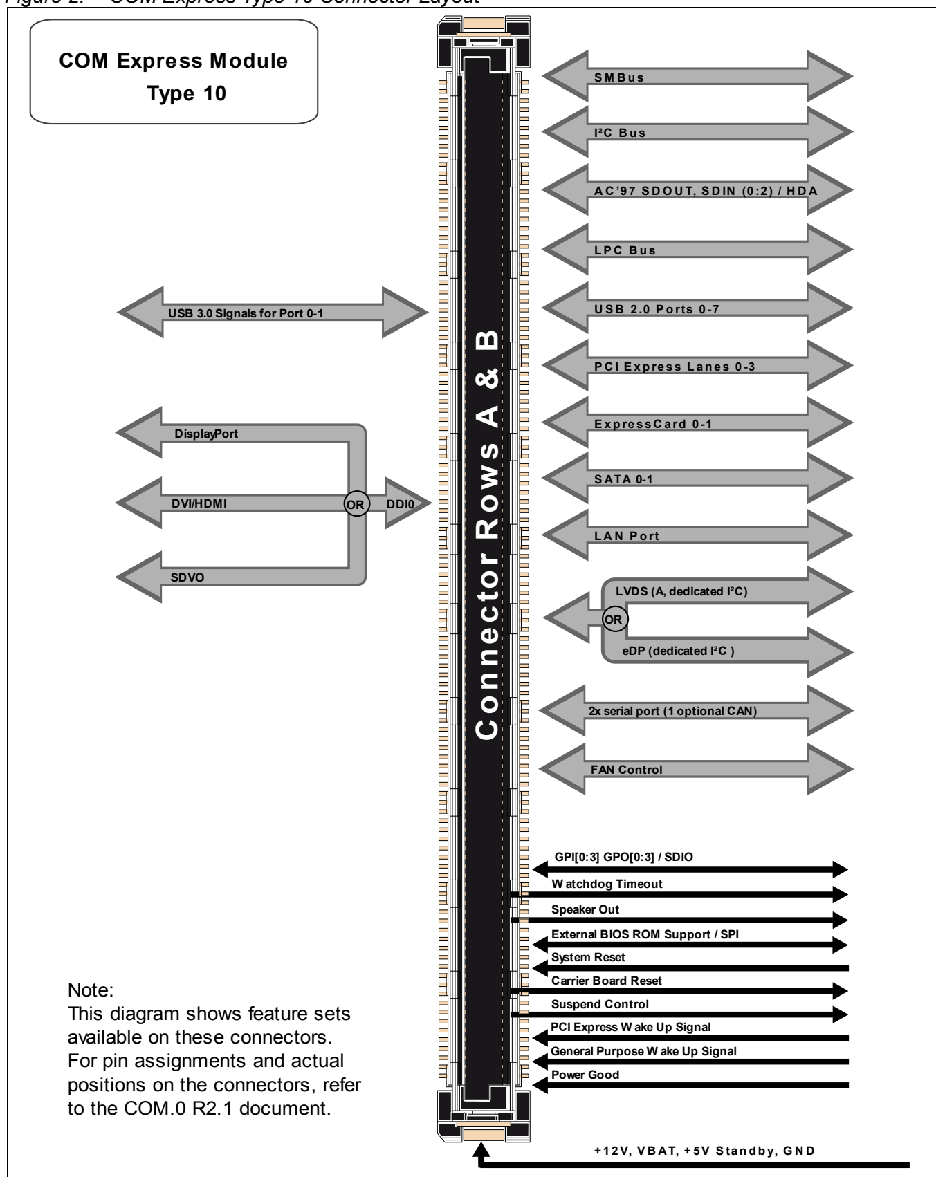
Figure 2: COM Express Type 10 Connector Layout
