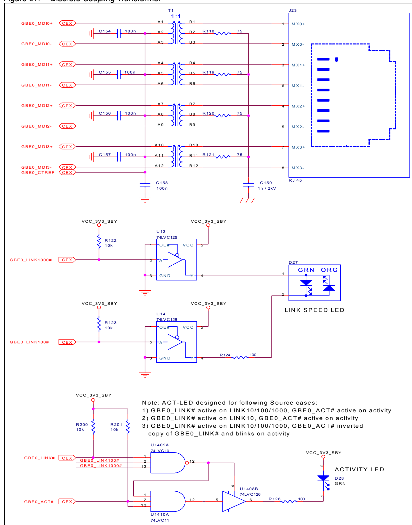
Figure 27: Discrete Coupling Transformer
