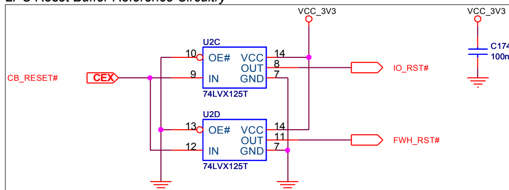
Figure 42: LPC Reset Buffer Reference Circuitry
