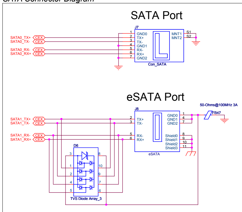
Figure 33: SATA Connector Diagram
