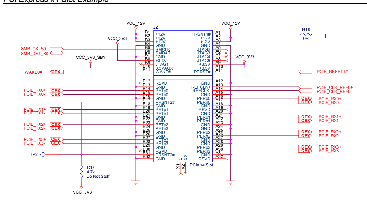
Figure 8: PCI Express x4 Slot Example
