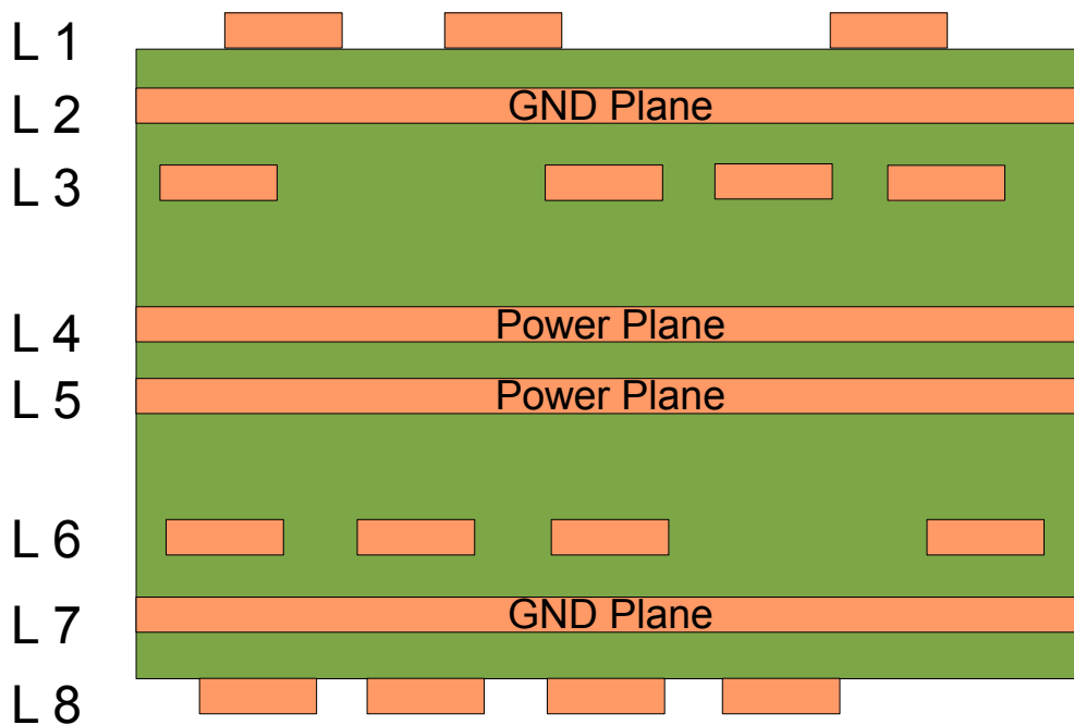
Figure 70: Eight-Layer Stack-up
