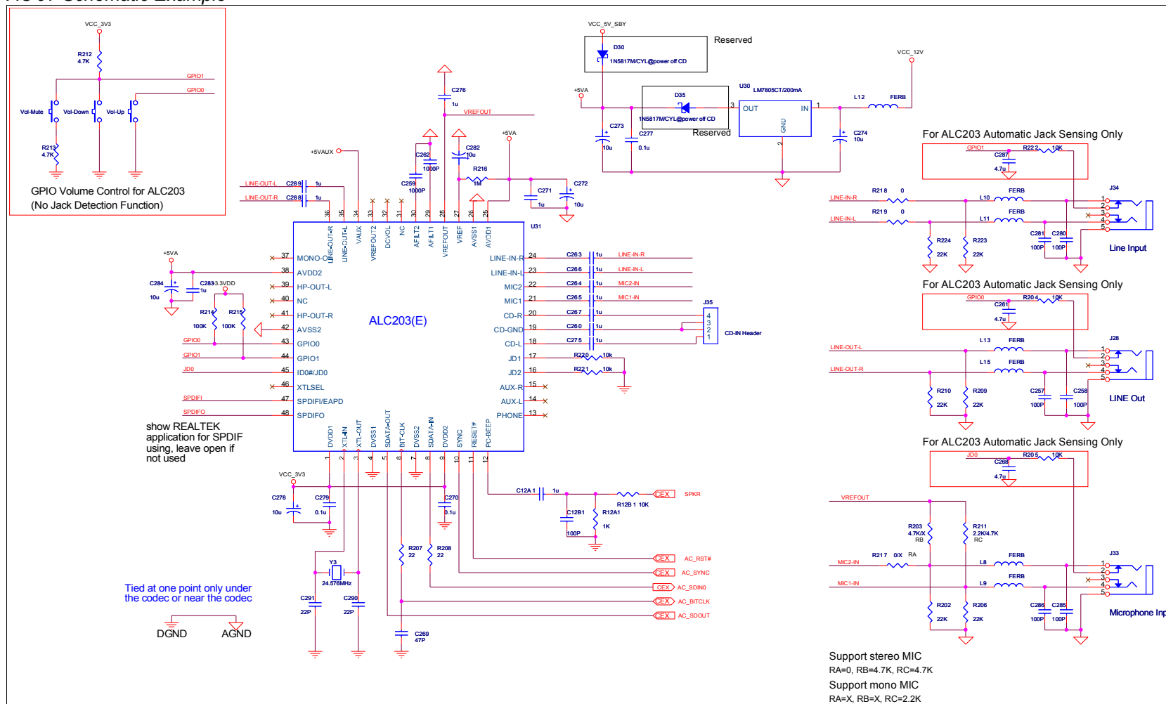
Figure 40: AC'97 Schematic Example
