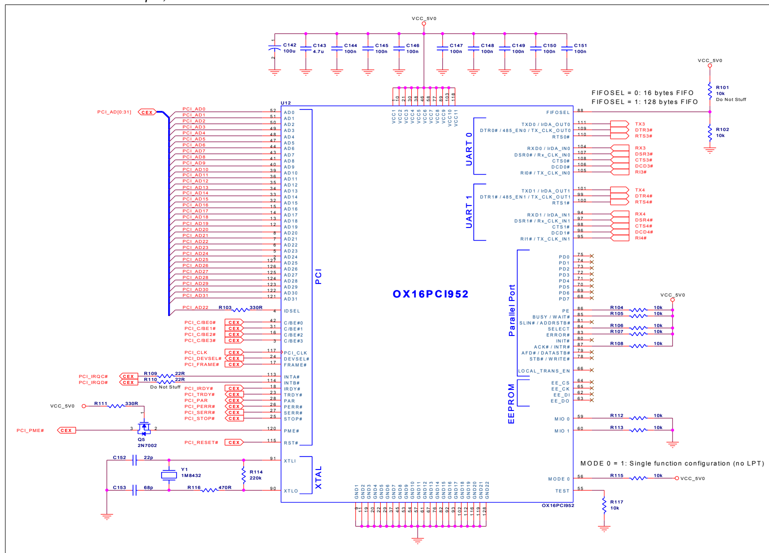
Figure 60: PCI Device Down Example; Dual UART
