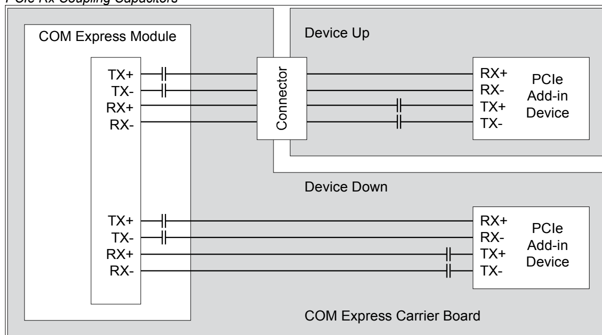
Figure 5: PCIe Rx Coupling Capacitors
