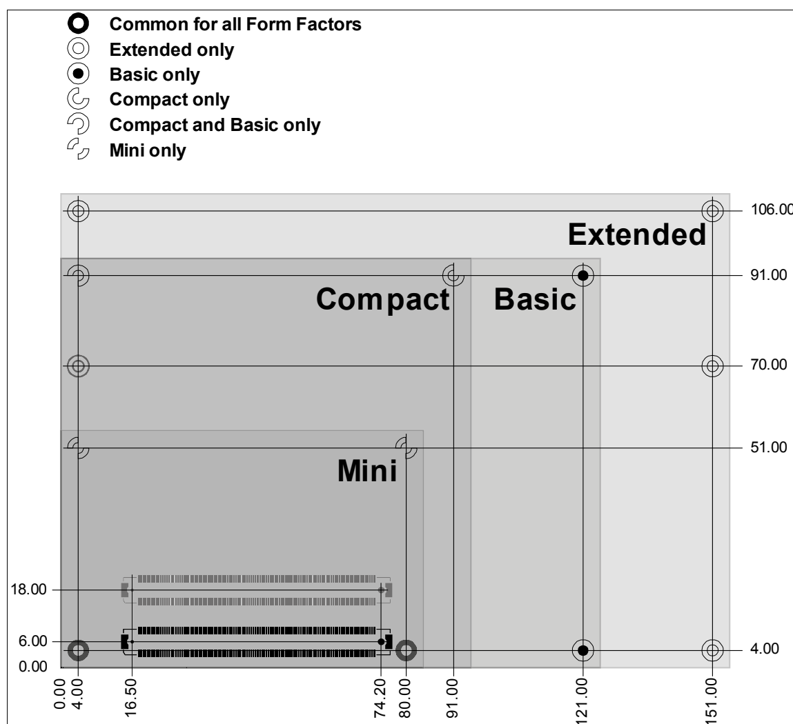
Figure 75: Mechanical comparison of available COM Express Form Factors
