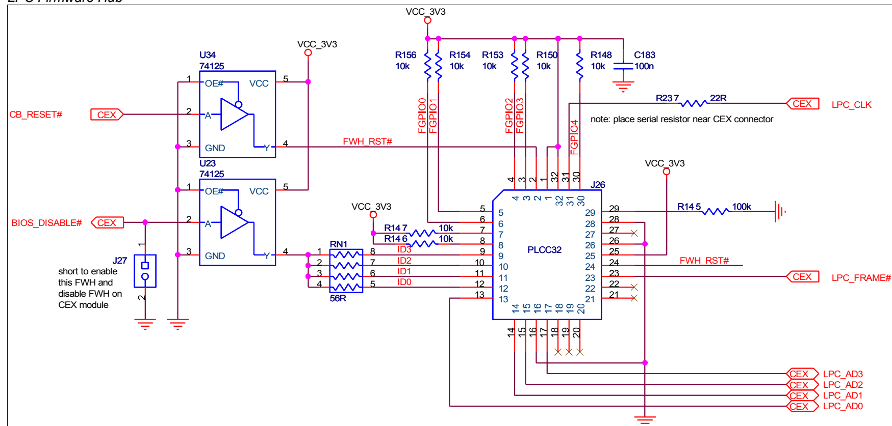
Figure 80: LPC Firmware Hub
