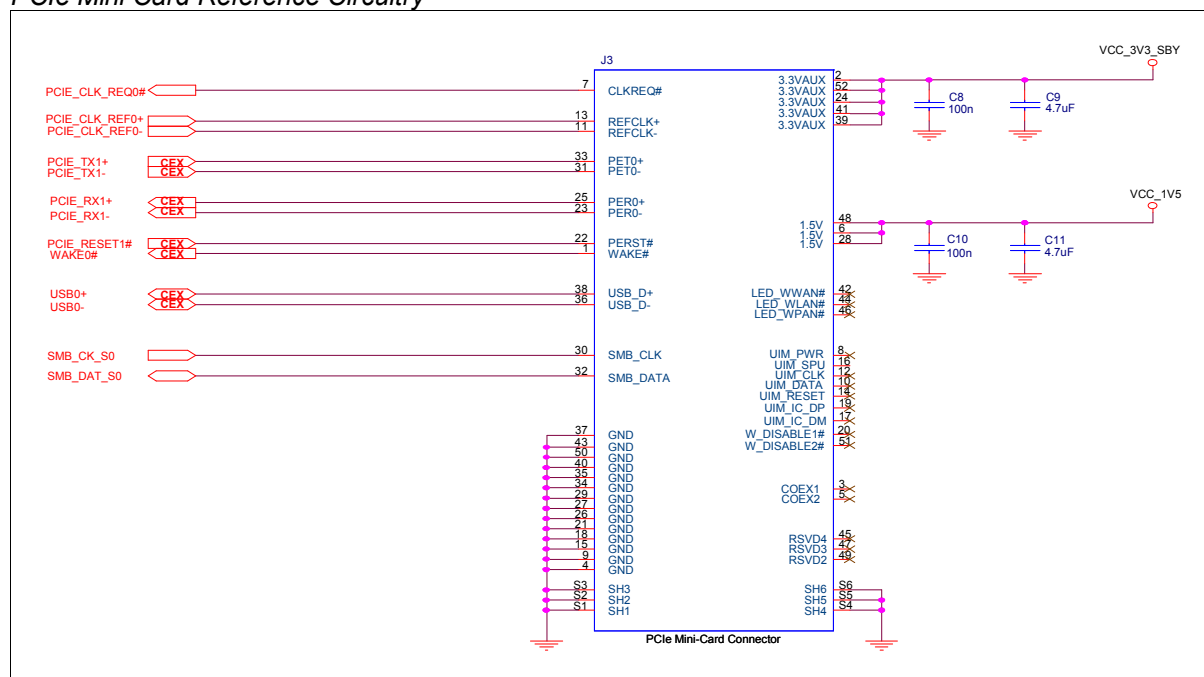
Figure 14: PCIe Mini Card Reference Circuitry
