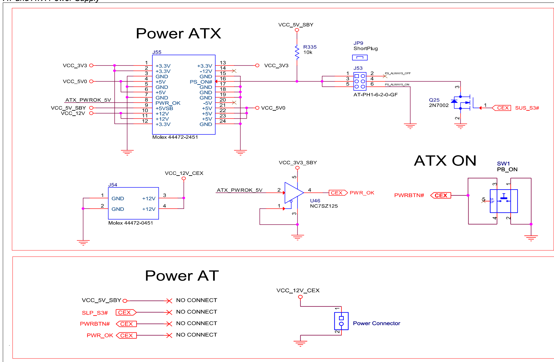
Figure 66: AT and ATX Power Supply
