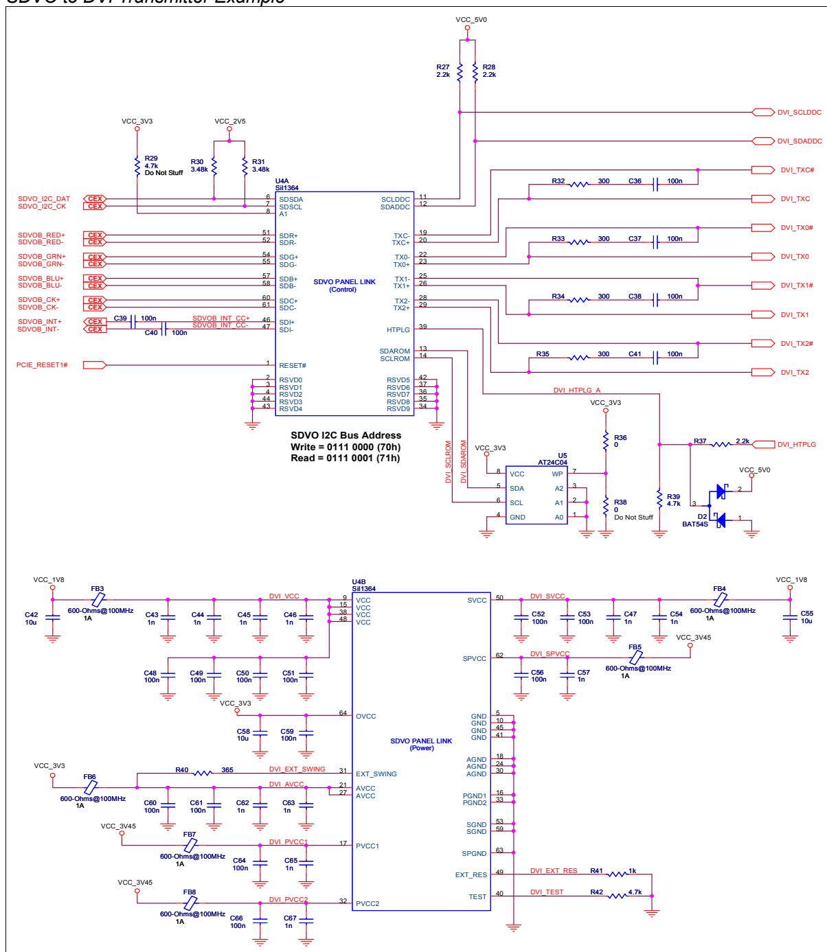
Figure 23: SDVO to DVI Transmitter Example
