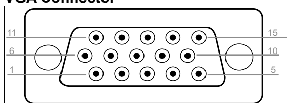
Figure 36: Female VGA Connector HDSUB15 for Carrier Board
