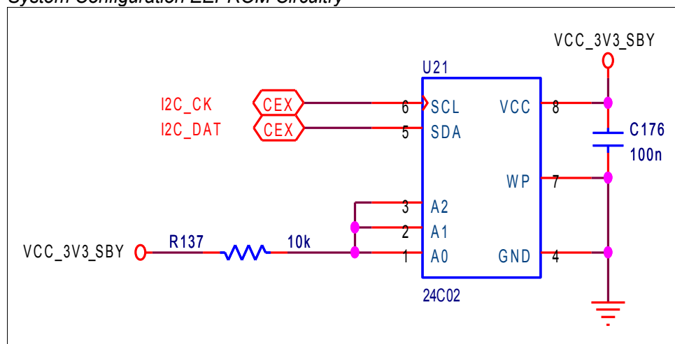
Figure 47: System Configuration EEPROM Circuitry
