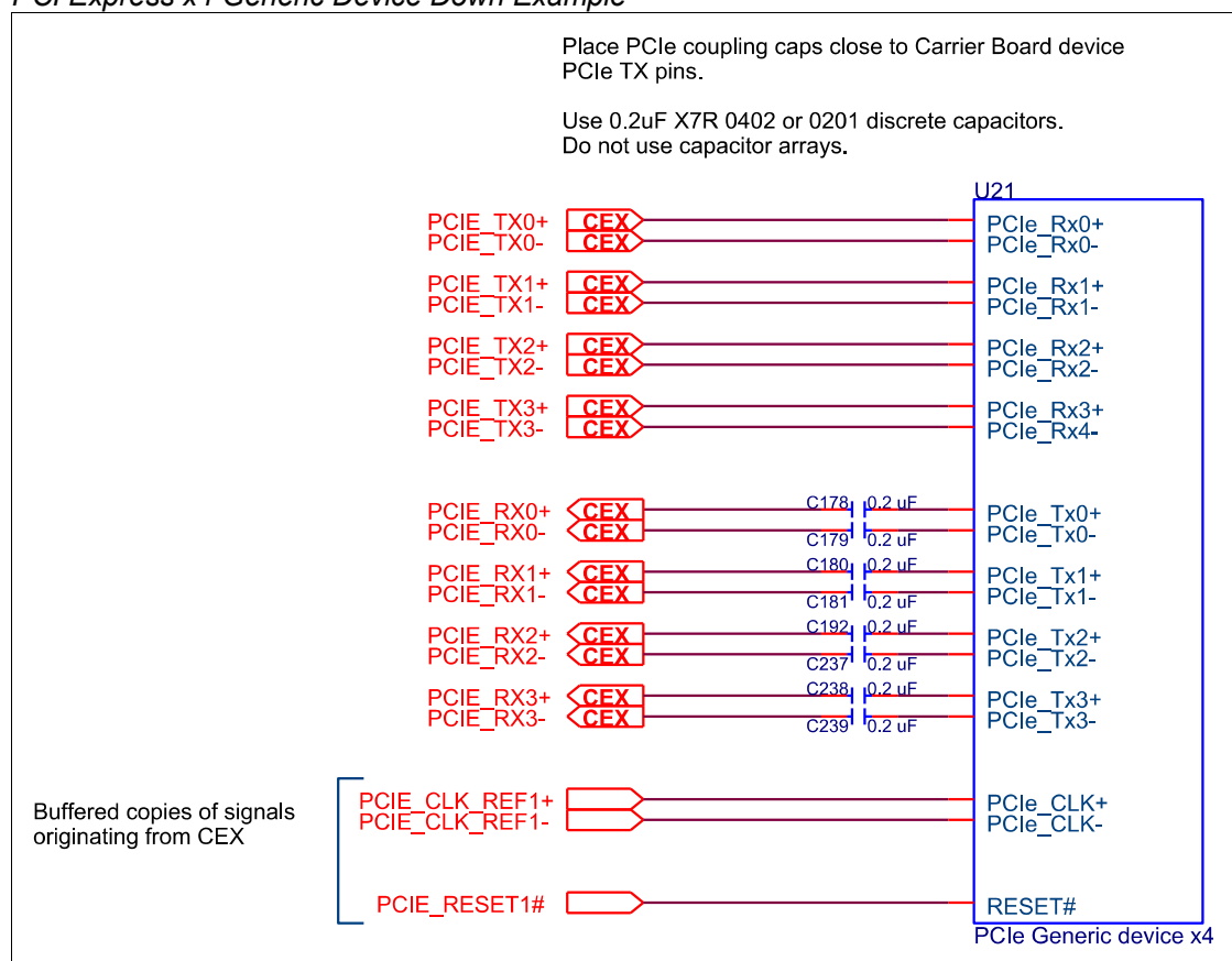
Figure 10: PCI Express x4 Generic Device Down Example
