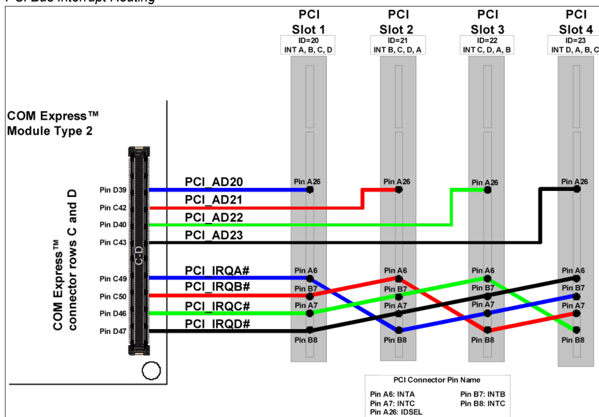
Figure 59: PCI Bus Interrupt Routing
