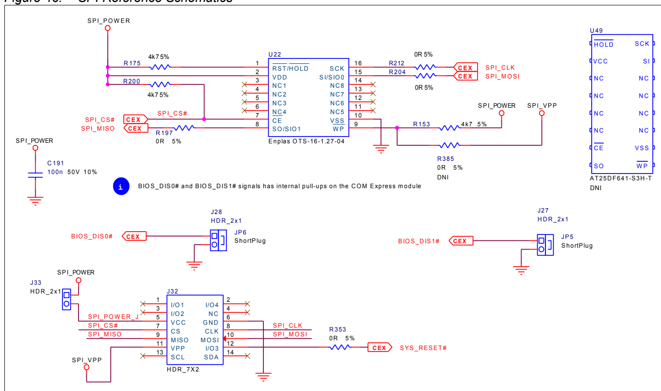
Figure 46: SPI Reference Schematics
