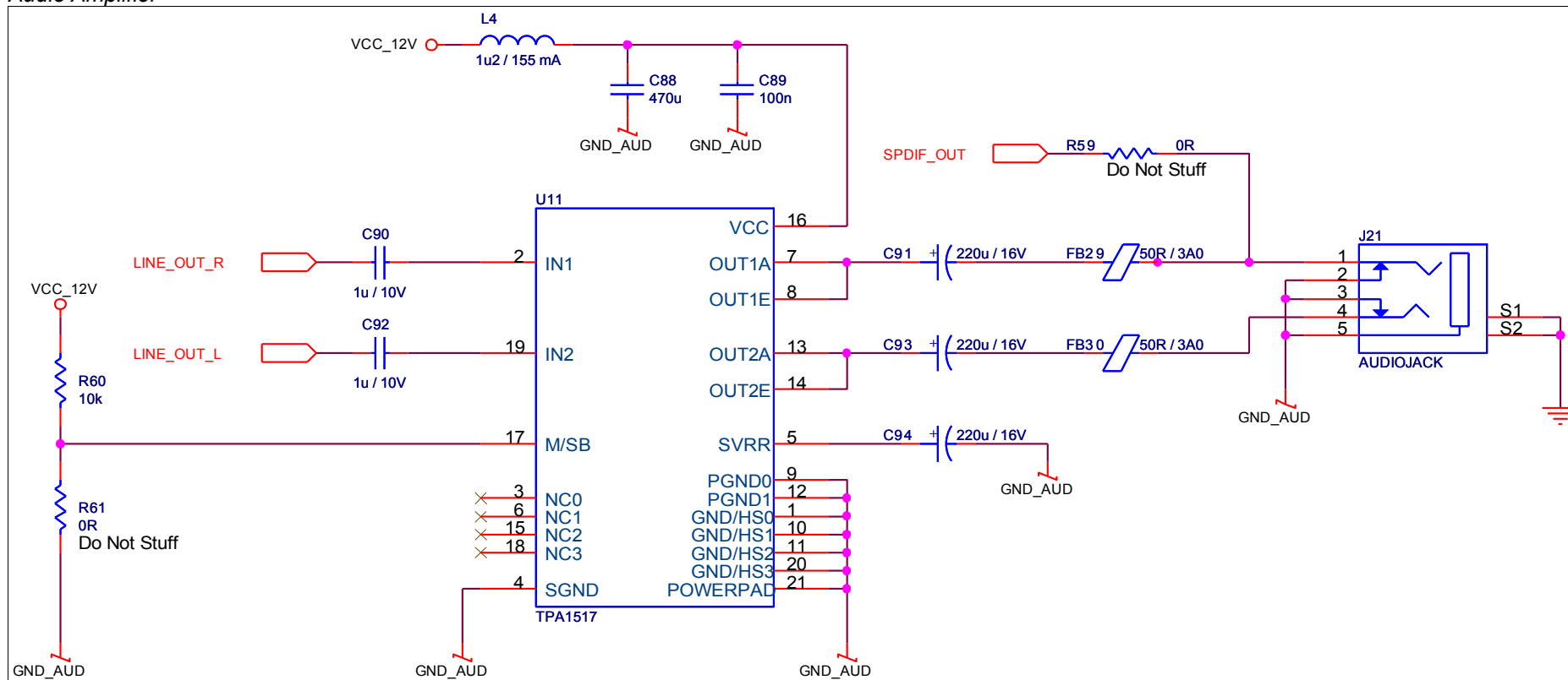
Figure 41: Audio Amplifier
